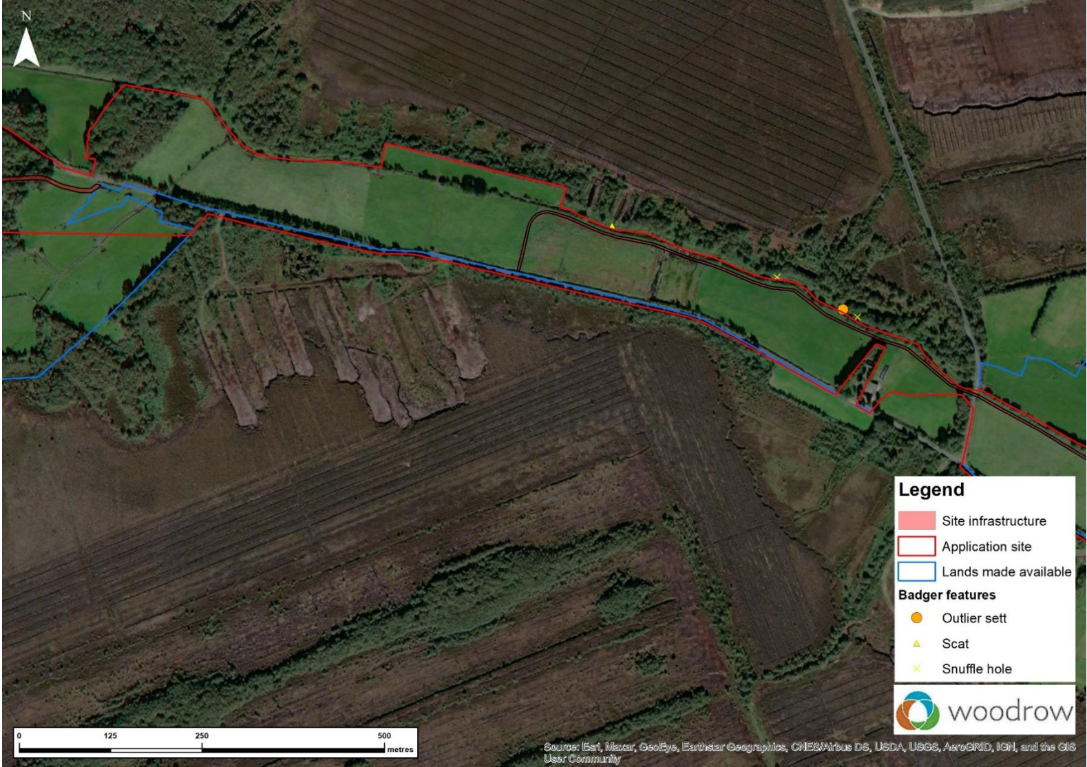
Figure A5.8.2: Badger activity along grid connection route
