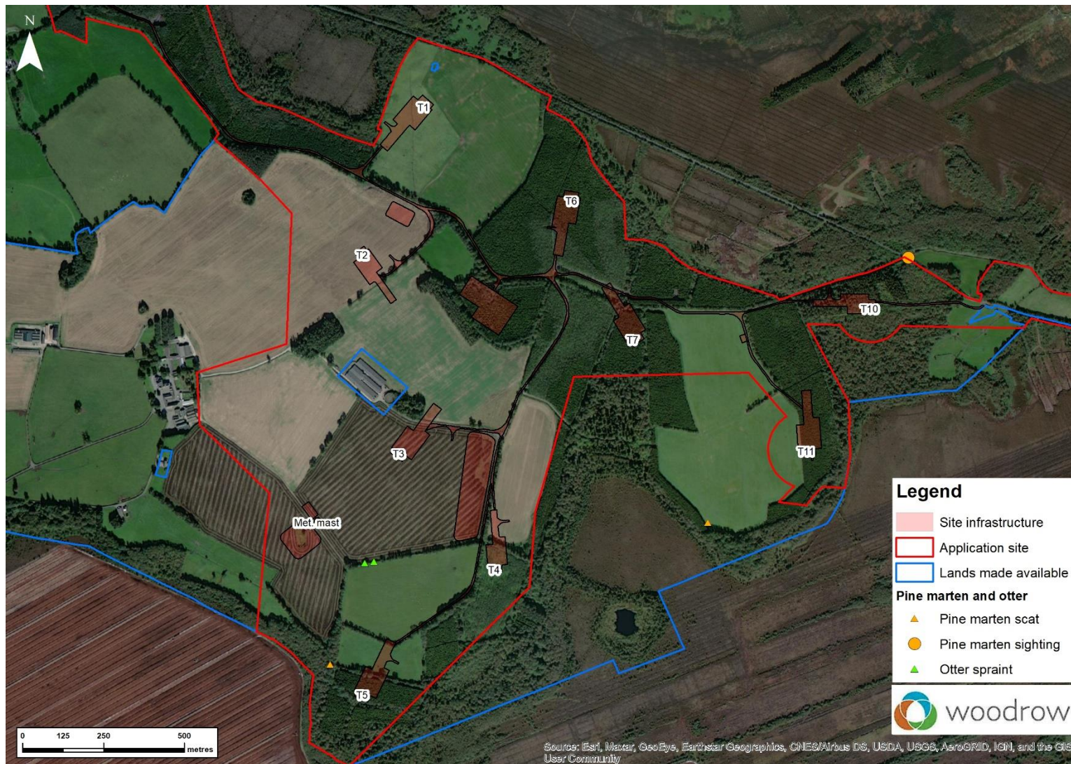
Figure A5.8.3: Otter and pine marten activity for proposed wind farm
